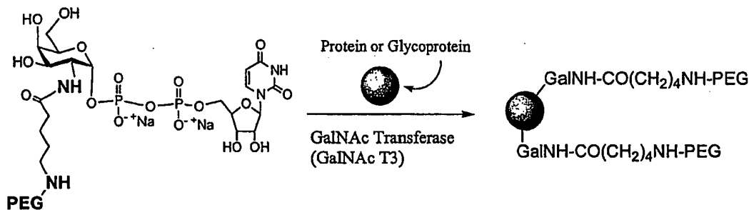
Scheme 14
